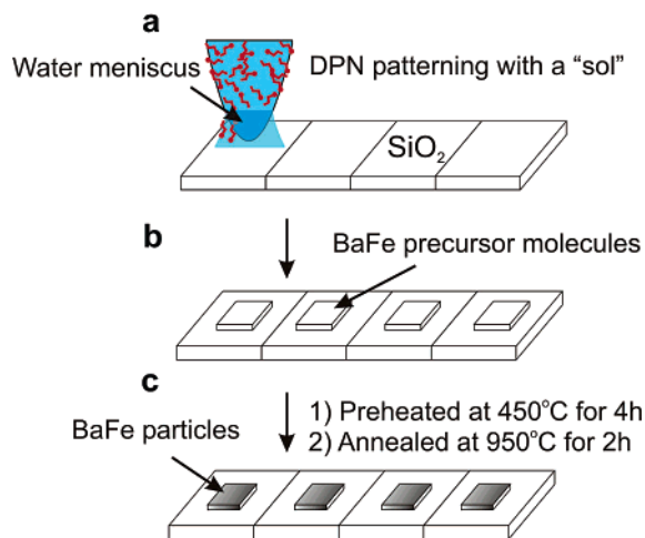
Figure 1. Schematic diagram depicting the patterning of magnetic BaFe nanostructures on silicon oxide. (a) An atomic force microscope (AFM) tip coated with a precursor solution of barium ferrite is brought into contact with the silicon oxide substrate. (b) The solution is transferred to the substrate as the tip is traversed across it. (c) Post-annealing yields the desired BaFe nanostructures.
